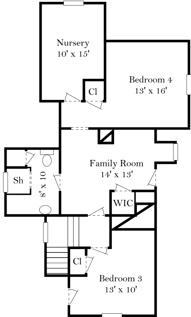
THIRD FLOOR
